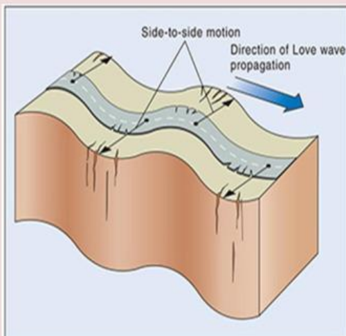
C Love wave
