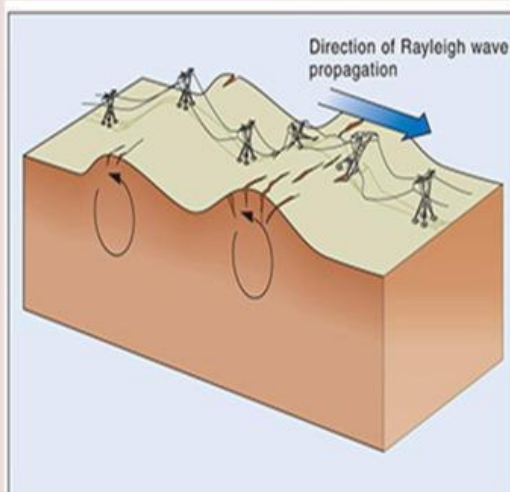
D Rayleigh wave
