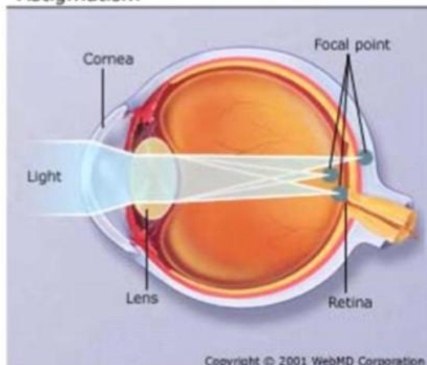
Astigmatism
