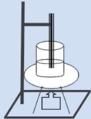
Gambar 3 Larutan C 6 H 8 O 6
