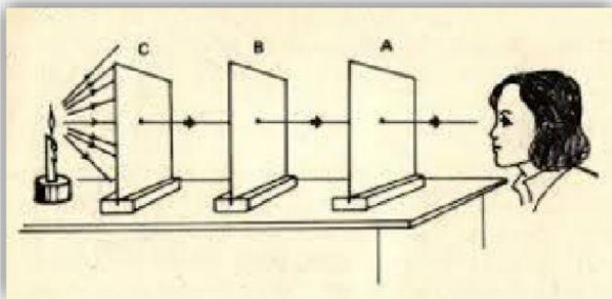
Gambar 4. Set Percobaan Perambatan Cahaya
