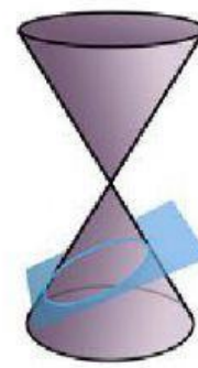
Elipse
