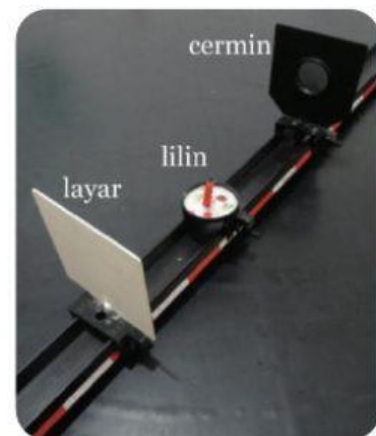
Gambar 9. Set percobaan cermin cekung
