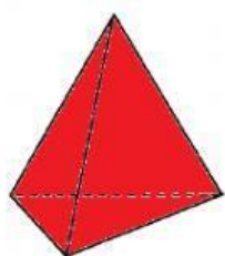
TETRAEDRO REGULARRA
