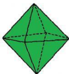
OCTAEDRO REGULAR
