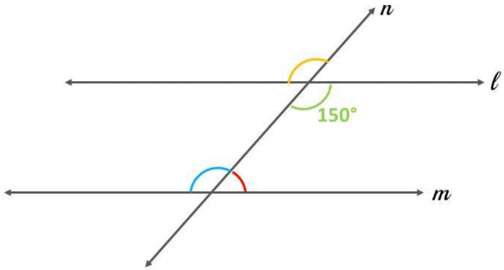
PARALLEL LINES AND TRANSVERSAL
