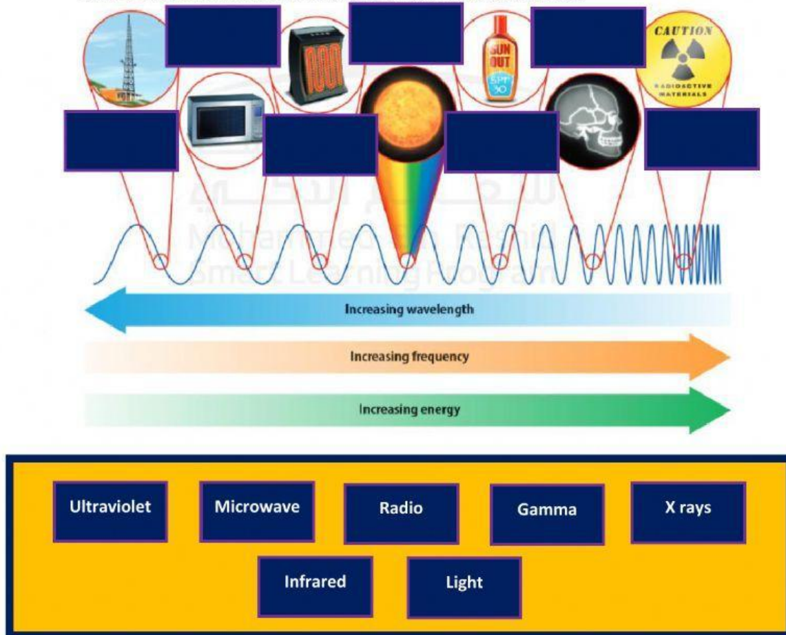
Figure 13 Electromagnetic waves have different wavelengths, frequencies, and energy.
