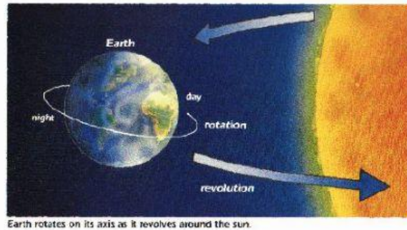
Earth rotates on its axis as it revolves around the sun.
