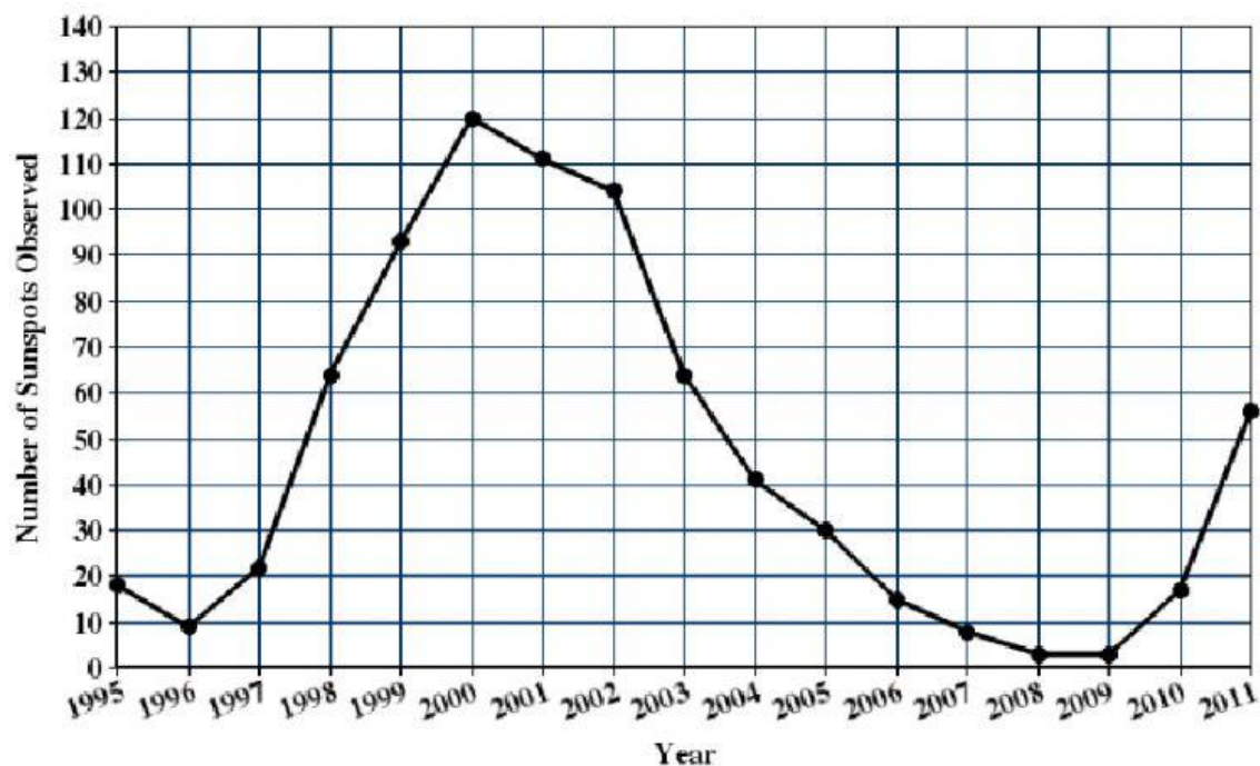
NUMBER OF SUNSPOTS OBSERVED PER YEAR
