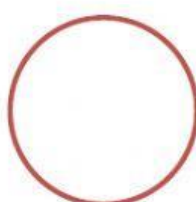
Screenshot 5
