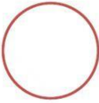
Screenshot 4
