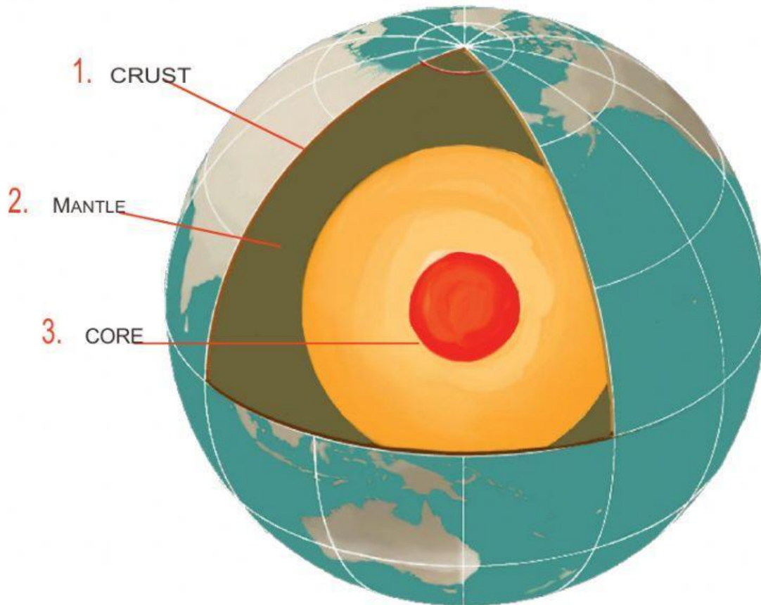
CRUST – MANTLE – CORE
