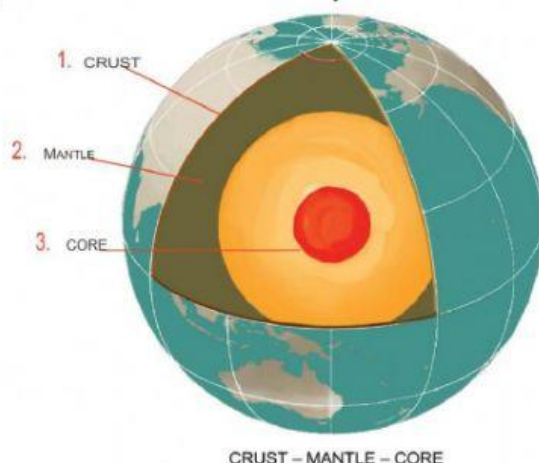
CRUST – MANTLE – CORE
