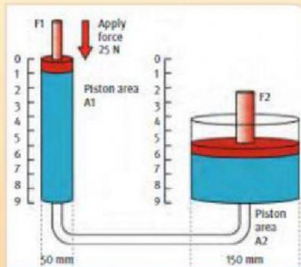
FIGURE 5 Hydraulic multiplication
