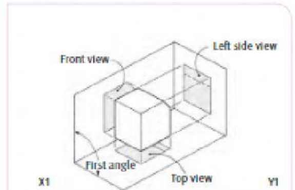
FIGURE 14 A first angle orthographic projection
