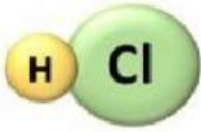
Molecule of hydrogen chloride
