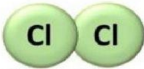
Molecule of chlorine
