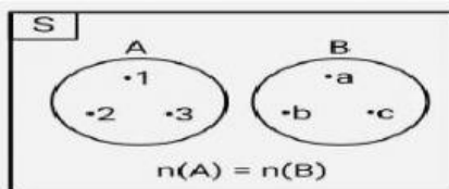
Diagram Venn Ekuivalen
