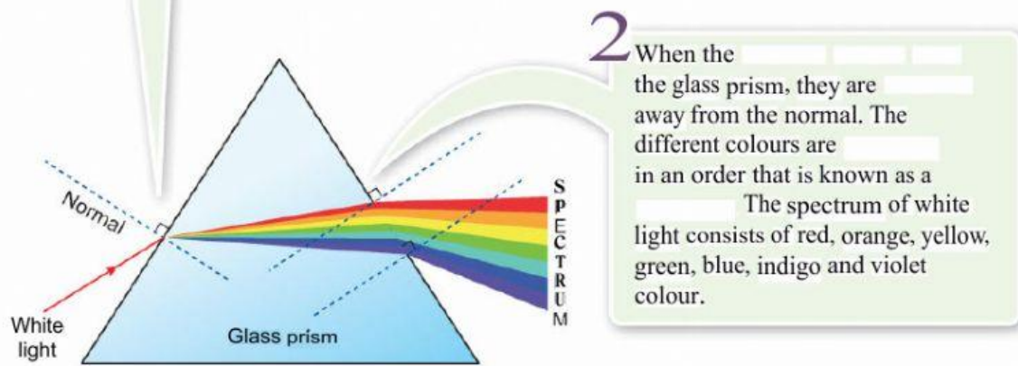
Figure 8.17 Dispersion of white light by a glass prism
