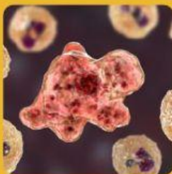
Amoeba
