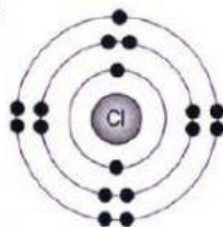
Atom klorin (2.8.7) Chlorine atom (2.8.7)
